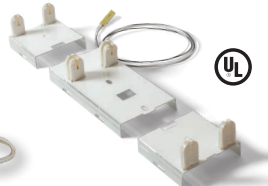
Pre-Wired 4-Foot Kit for two (2) Single-End Powered T8 LED Lamps Part Number: 14073
